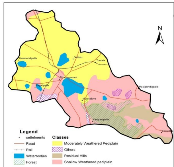
Figure 5: Hydro-geomorphology of the study area
