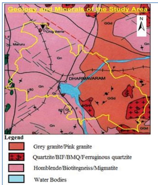
Figure 6: Geology and minerals of the study area
