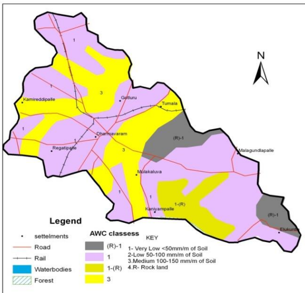
Figure 4: Water capacity of the study area
