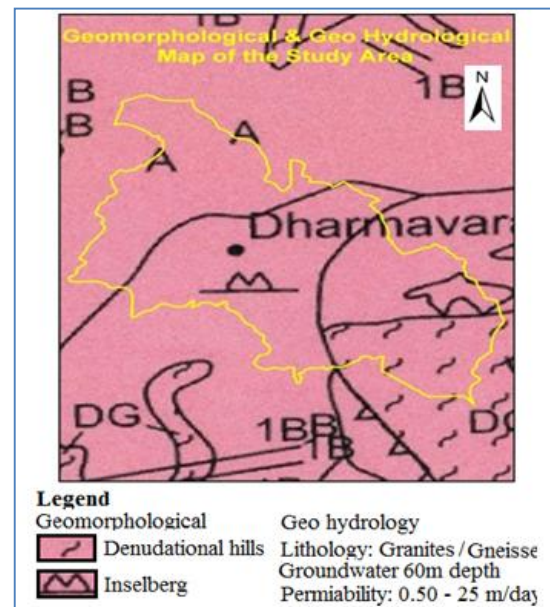
Figure 7: Geomorphology & geo-hydrology
